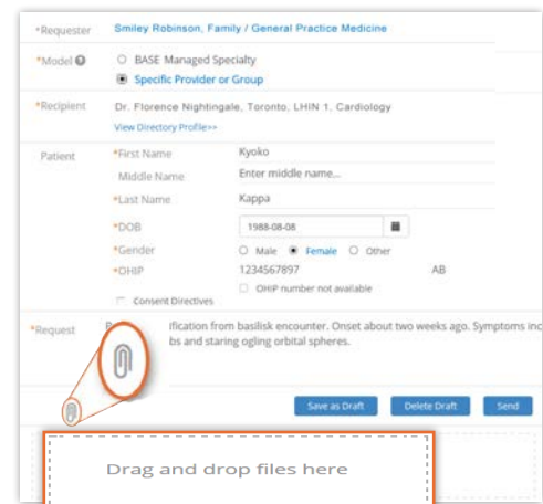
Figure 11: Two methods to attach files
